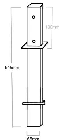
In ground fixing post detail
