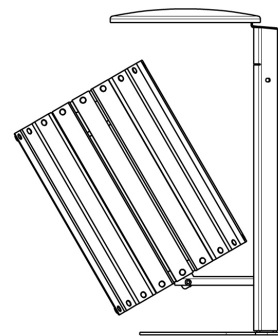
Surface fixed in tilt position
