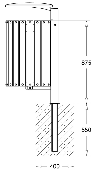
In-ground fixed
